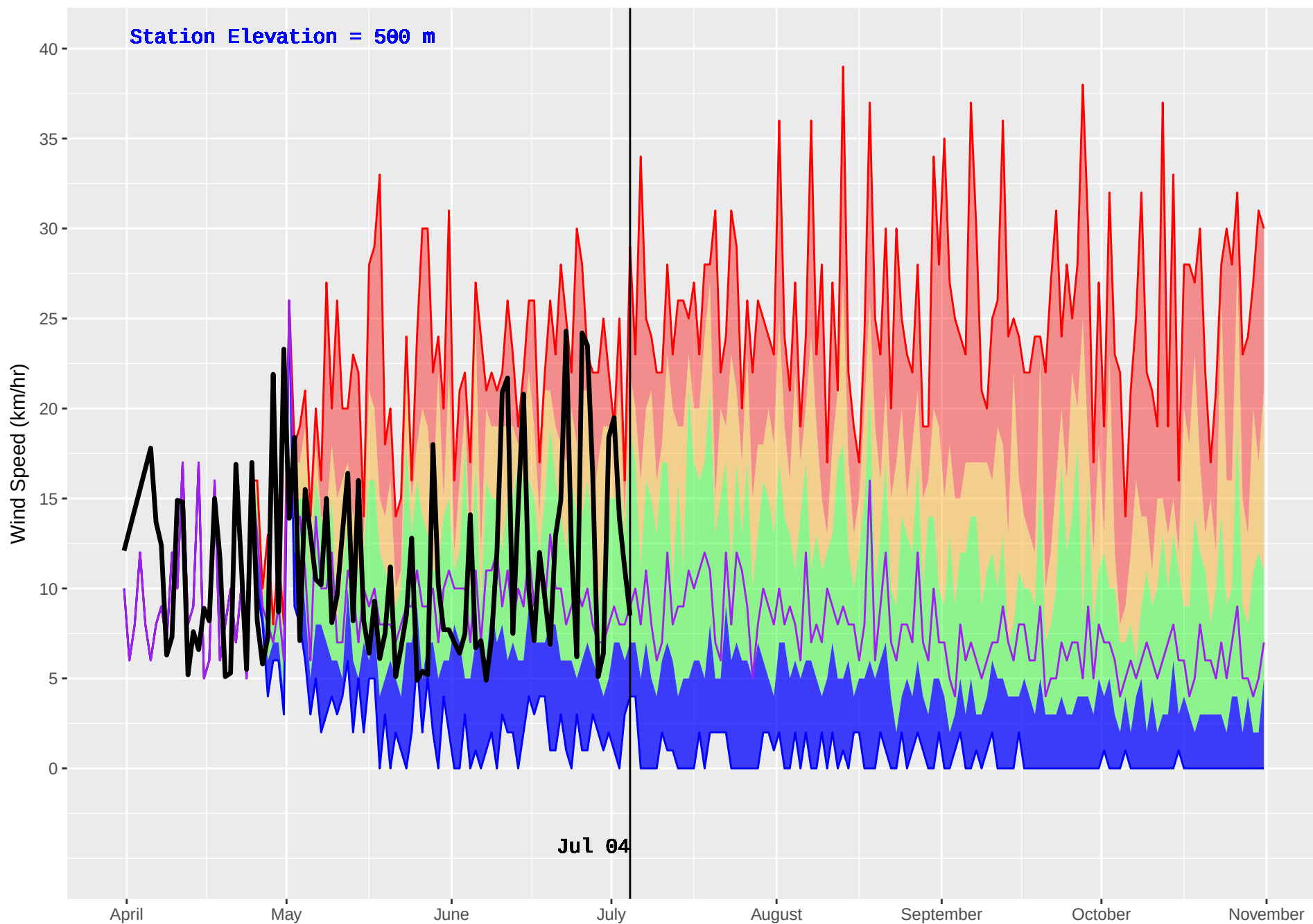
CRANBERRY (433) : Historical (1995–2016) and Current (2018) Noon Wind Speed
