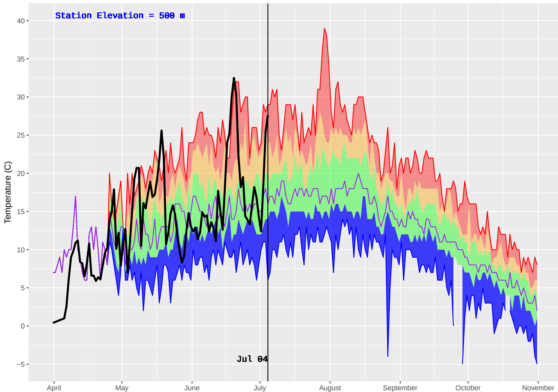
CRANBERRY (433) : Historical (1995–2016) and Current (2018) Noon Temperature
